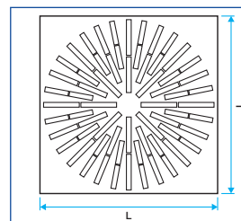
Dimension 825 x 825
